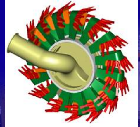
DREDGING WHEEL
